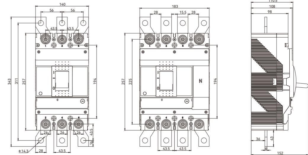
SGM6/6s/6sm-400A(Me) 3 POLES & 4 POLES
