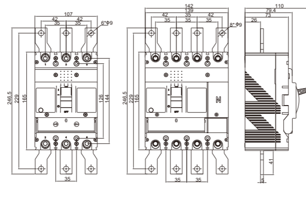
SGM6/6s/6sm-250A(H*) 3 POLES & 4 POLES
