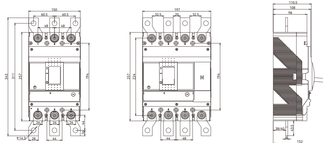
SGM6/6s/6sm/6E-400A/630A 3 POLES & 4 POLES
