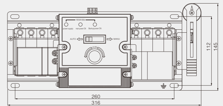
Total height: 123mm
