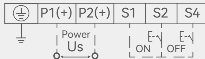
Electrical wiring diagram
