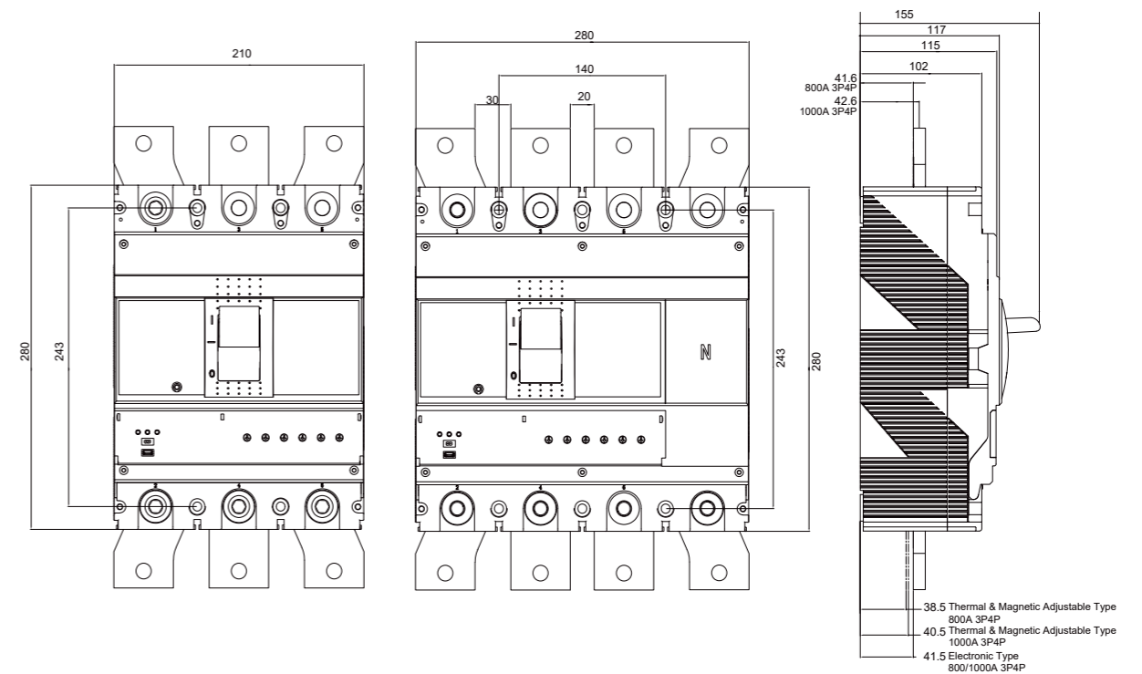
SGM6/6s/6sm/6E-800/1000A 3 POLES & 4 POLES
