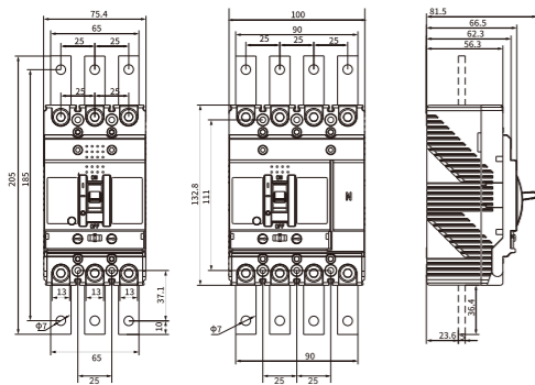
SGM6/6s/6sm/6E-250A 3 POLES & 4 POLES
