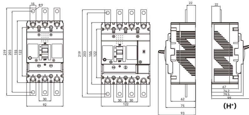
SGM6/6s/6sm-250A(H*) 3 POLES & 4 POLES
